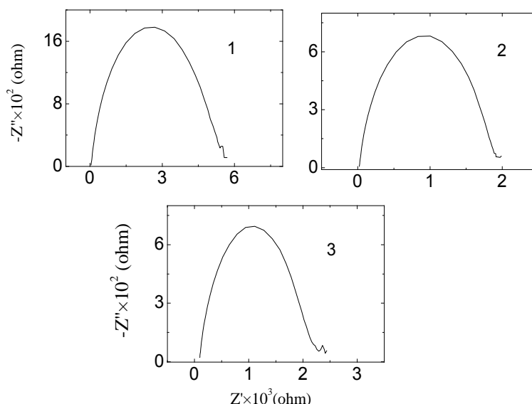
Fig. 4 – EIS Nyquist plots of DSSCs sensitized by (1) safflower, (2) Medicago sativa and (3) Ros marinus under an illumination of 100 \text{ mW/cm}^2 and -0.7 \text{ V} applied voltages
