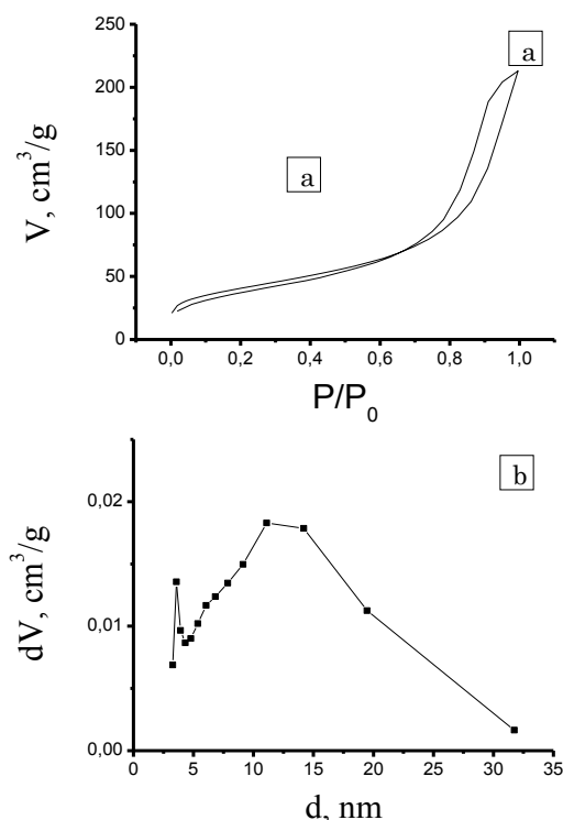
Fig. 2 – N 2 isotherms (a) and pore-size distribution for TiO 2 doped with Nb (b)
