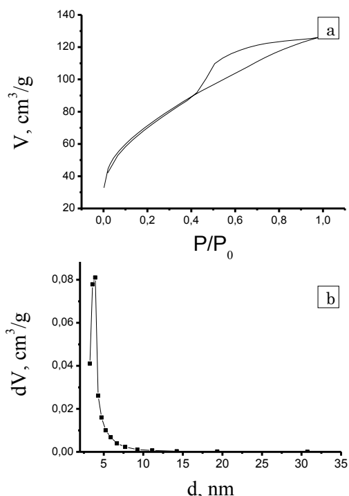
Fig. 3 – N 2 isotherms of nitrogen (a) and pore size distribution for Zr-doped TiO 2 (b)
