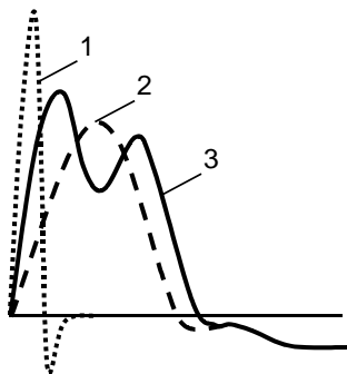
Fig. 2 – Dependency of the shape of the pulse generated in the deformation zone on the type of the shock system (Table 1)
