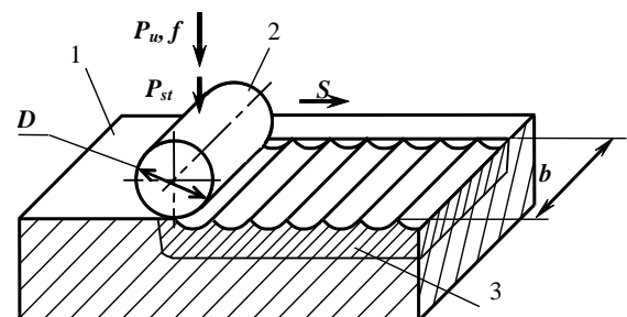
Fig. 3 – Diagram showing making impressions on a workpiece plane surface by a core roller in the process of static-pulse treatment (1 – specimen, 2 – core roller, 3 – hardened area): P_u – impulsive load, f – impulse frequency, P_{st} – static load, S – workpiece feeding speed relative to the roller, D – roller diameter, b – roller width
