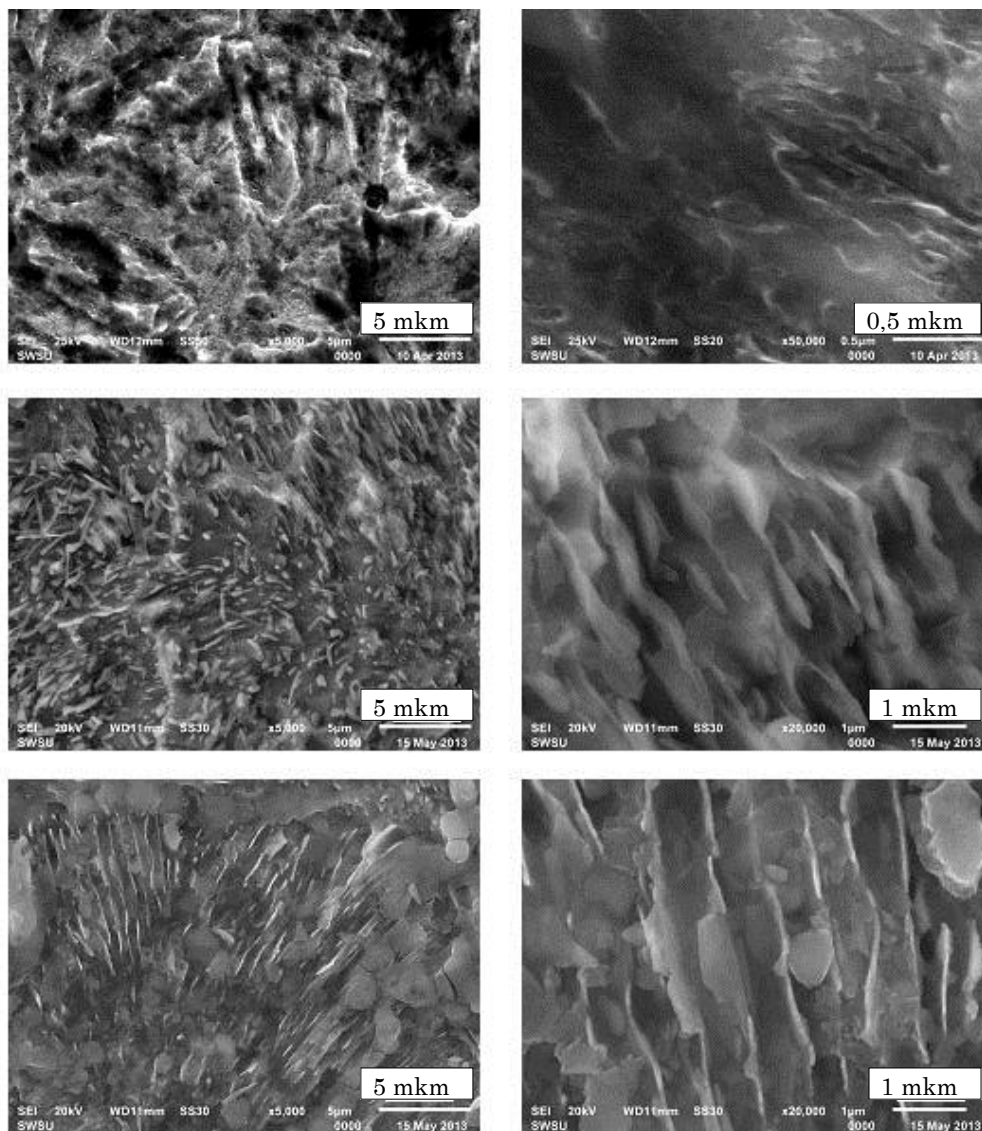
Fig. 4 – SEM images of specimen surfaces (steel 45) after an impact made by deformation shock waves with decreasing displacement in relation to each other (top-down)
