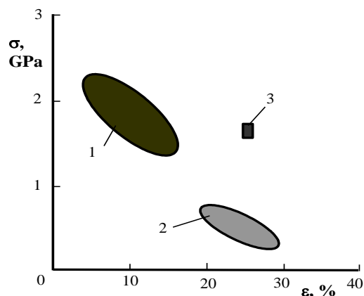
Fig. 1 – Correlation between steel hardness and plasticity shown by the curve of relationship of ultimate strength \sigma and percentage extension \varepsilon : 1 – high-strength steels, 2 – low-carbon steels, 3 – nanocrystal steel [3]
