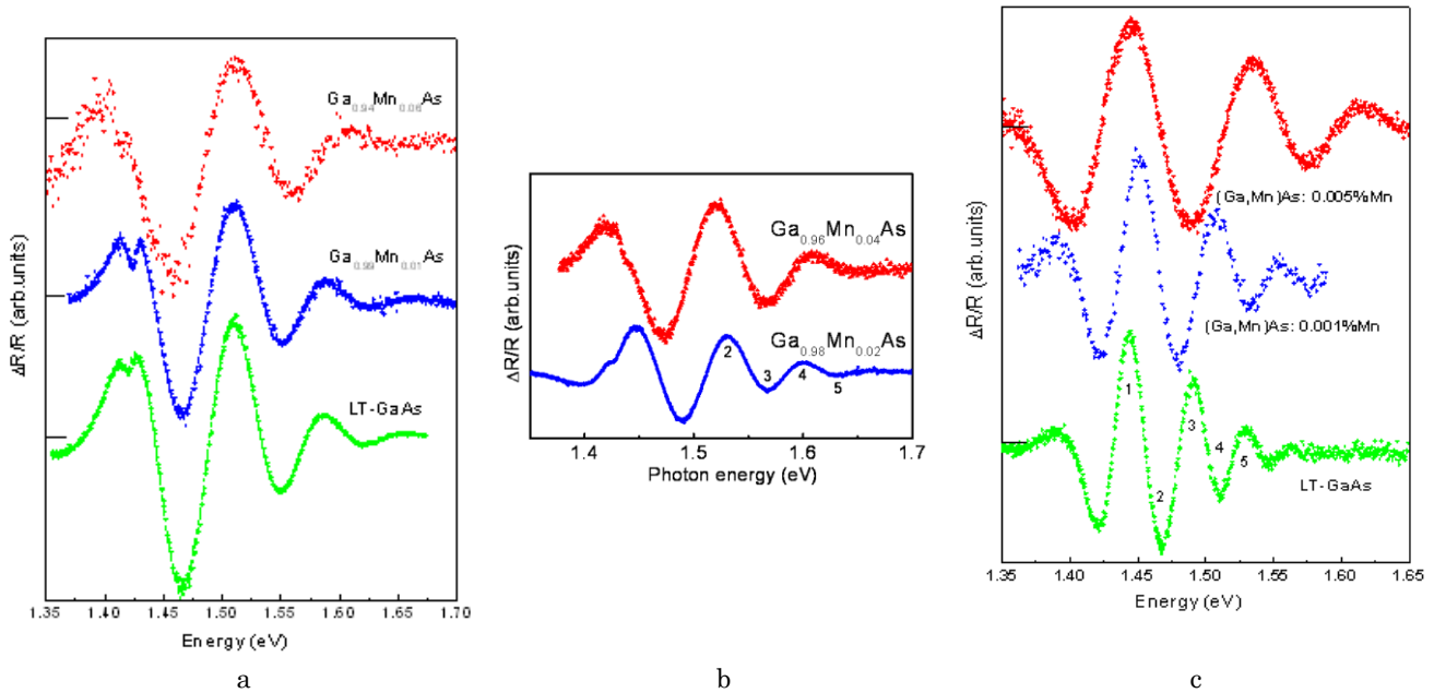
Fig. 3 – Sequence of the photoreflectance spectra for the LT-GaAs, (Ga,Mn)As films epitaxially grown on GaAs substrate: (a) 230 nm LT-GaAs, Ga 0.98 Mn 0.01 As, and Ga 0.94 Mn 0.06 As; (b) 300 nm Ga 0.98 Mn 0.02 As and Ga 0.96 Mn 0.04 As; (c) 800-700 nm LT-GaAs, (Ga, Mn)As: 0.001% Mn, and (Ga, Mn)As: 0.005% Mn. The curves have been vertically offset for clarity
