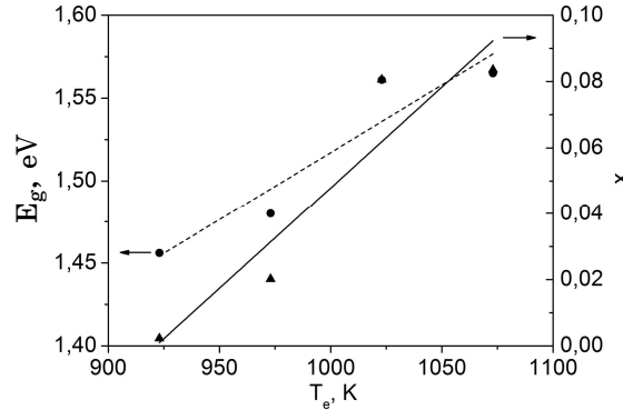
Fig. 6 – Dependence of the BG E_g and manganese content x of \text{Cd}_{1-x}\text{Mn}_x\text{Te} triple compound in the films on the evaporation temperature T_e of the material
