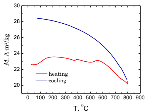
Fig. 6 – Temperature dependence of the magnetization of nanocomposites NiCo / C synthesized at 800 °C
