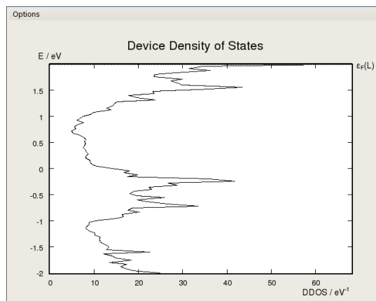
Fig. 7 – Density of states of spinel LiMn 1.5 Ni 0.5 O 4
